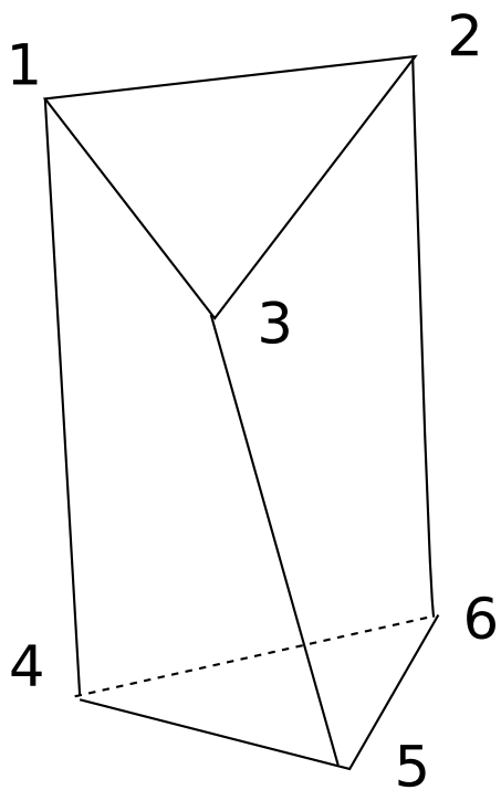
Prism
