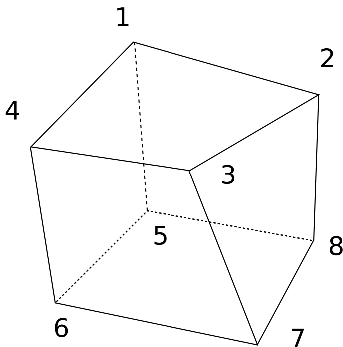
Hexahedron
